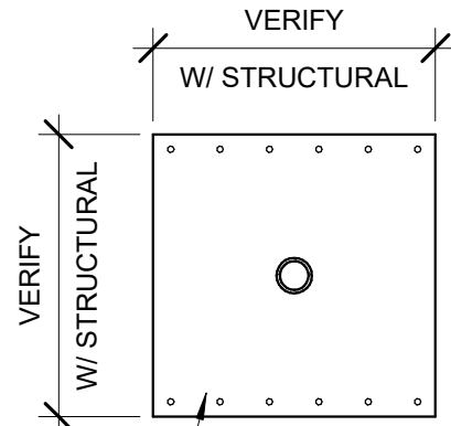
PLAN VIEW OF STEEL PLATE
